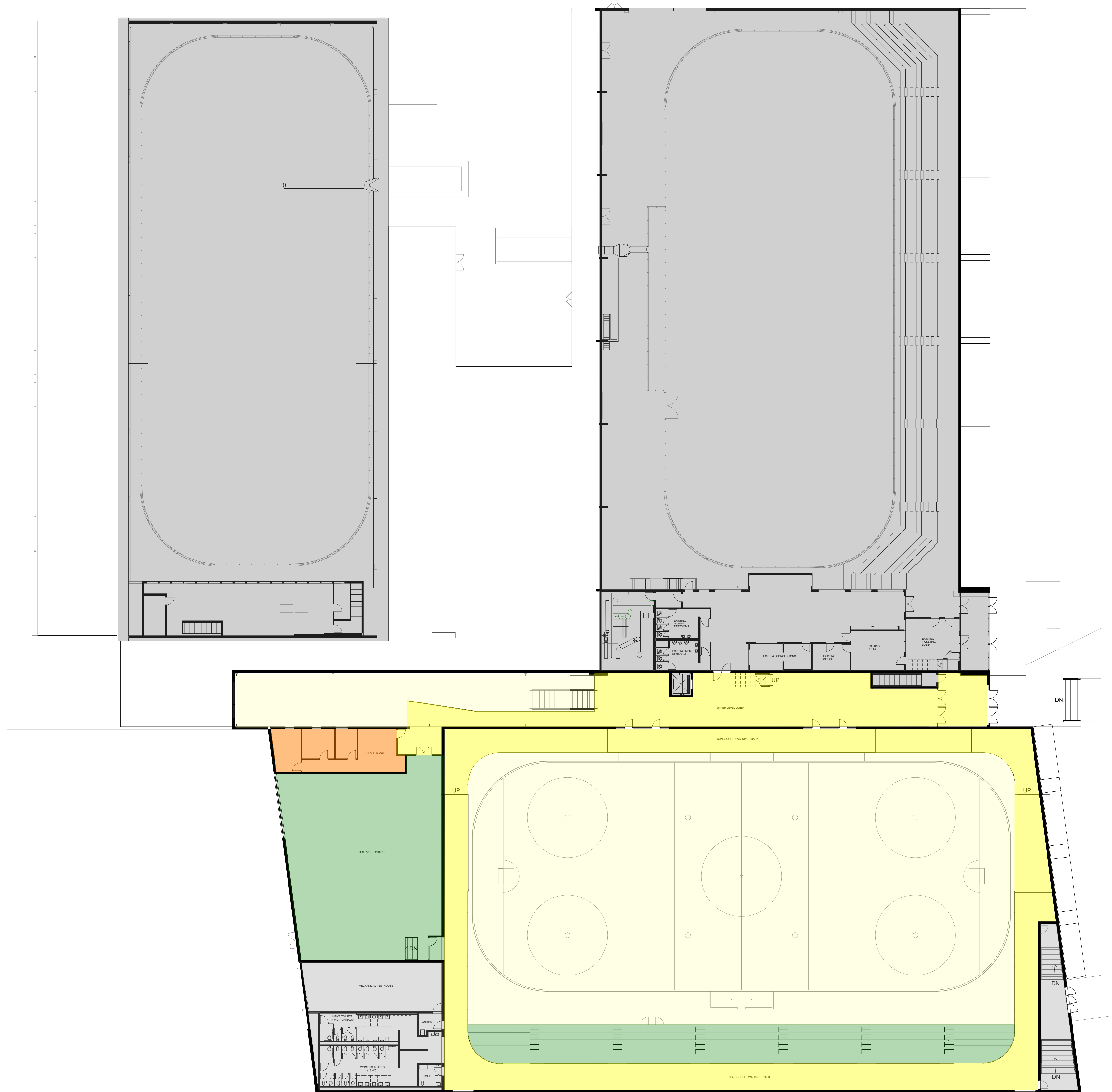
① FLOOR PLAN - Proposed Upper Level 1/16" = 1'-0"
