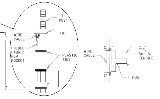
FABRIC/CABLE/POST CONNECTION
