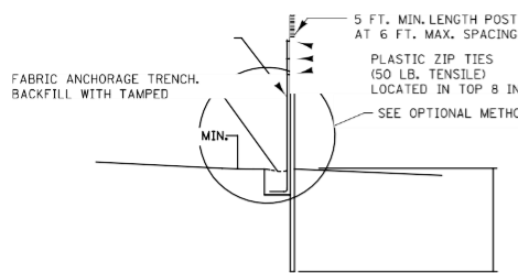
SILT FENCE TYPE HI @ HAND INSTALLED
