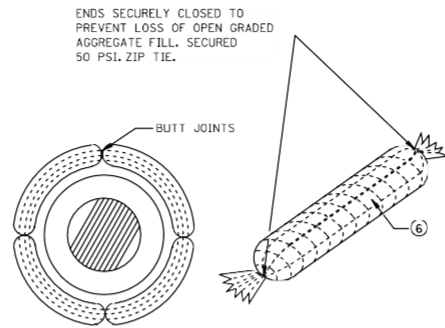
ROCK LOG/COMPOST LOG
