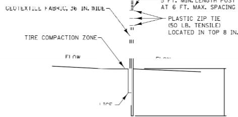
SILT FENCE TYPE MS @ DMA CHINE SLICED
