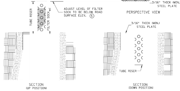
POP-UP HEAD
