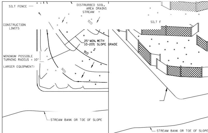
INSTALLATION AT BRIDGE EMBANKMENT ADJACENT TO WATER
