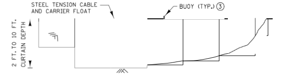
FRONT VIEW FOR FLOTATION SILT CURTAIN
