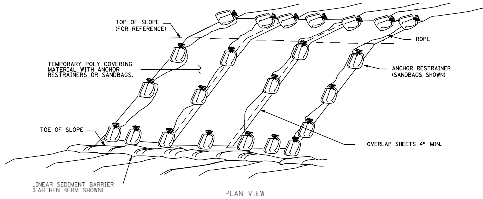
TEMPORARY POLY COVER ON SLOPE
