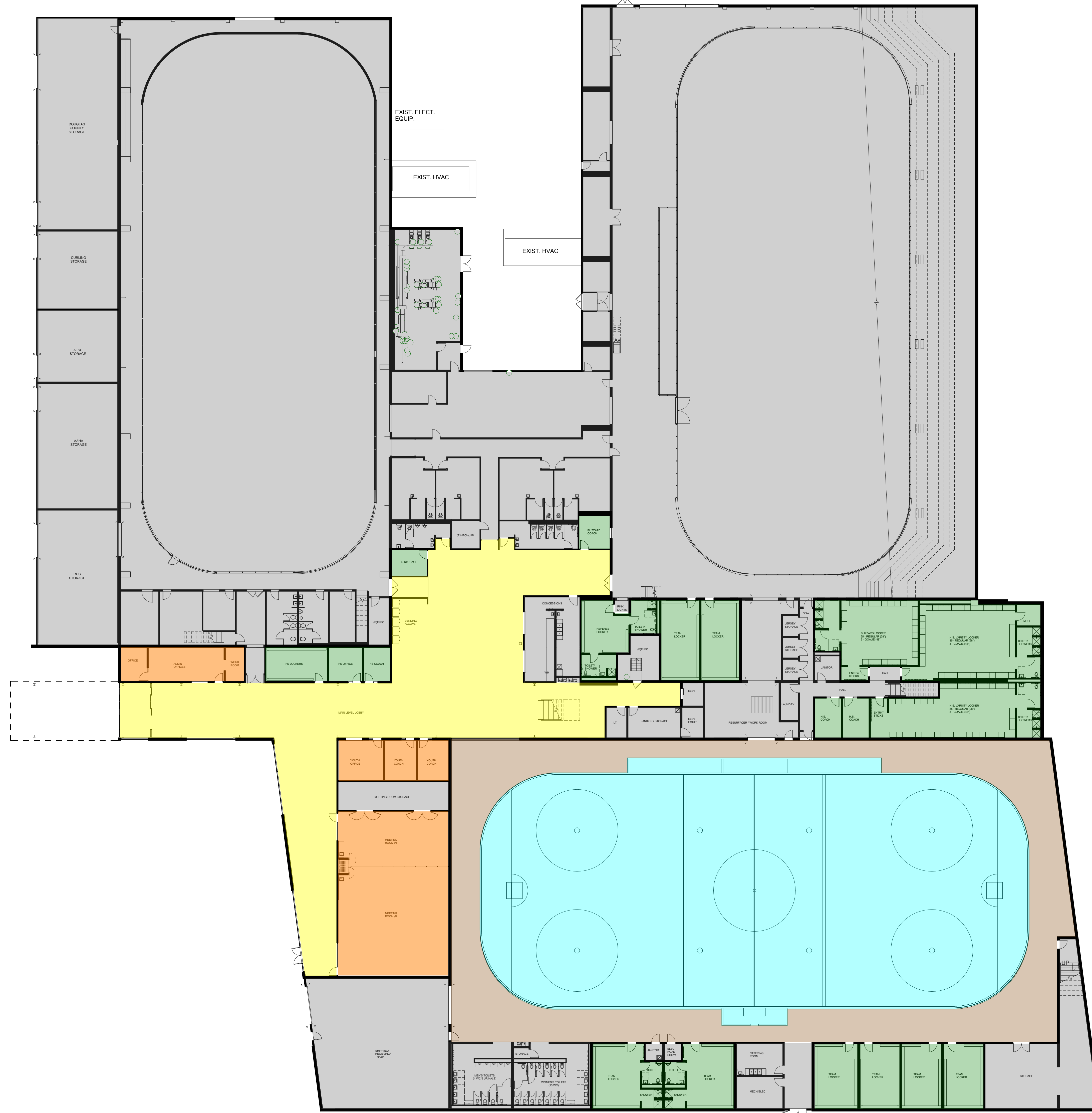
1 FLOOR PLAN - Proposed Main Level 1/16" = 1'-0"
